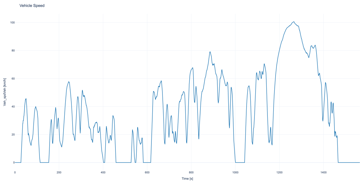
Figure: Vehicle Speed
