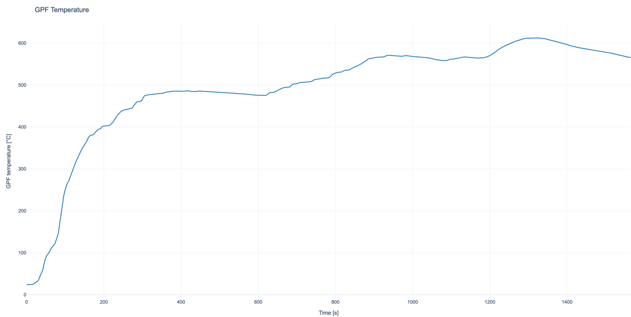
Figure: GPF Temperature
