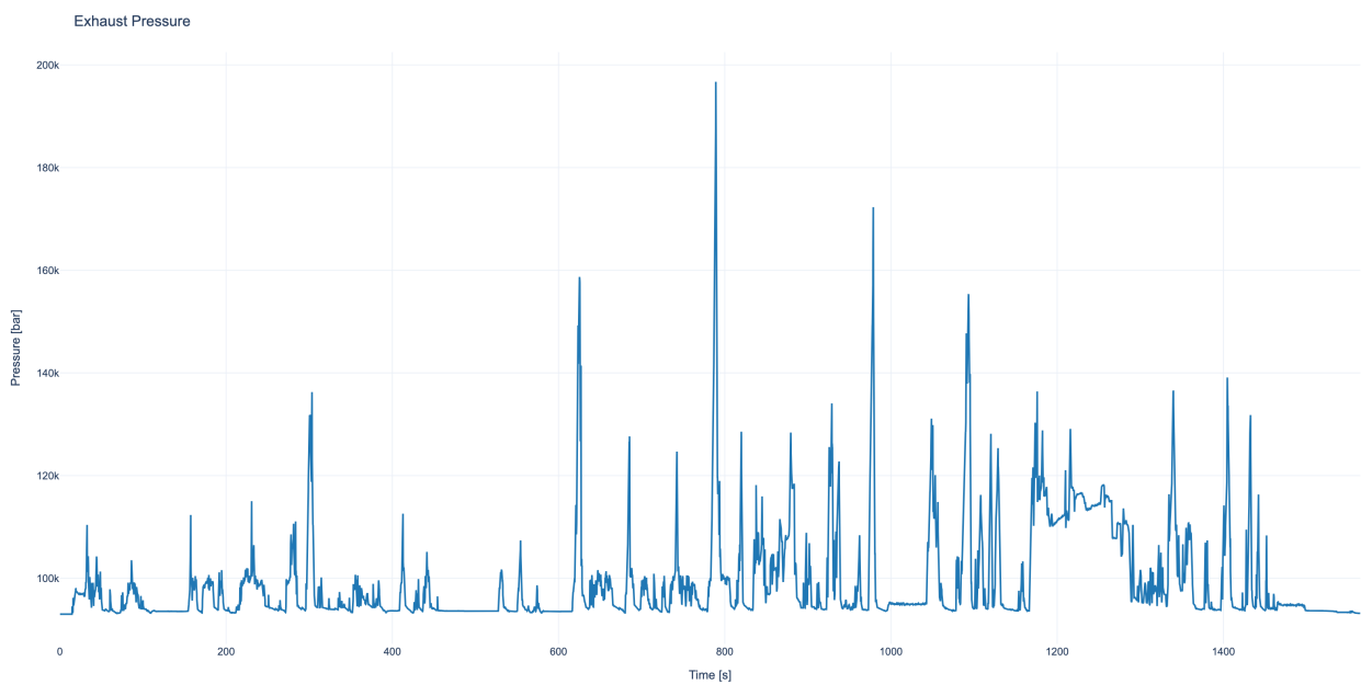
Figure: Exhaust Pressure
