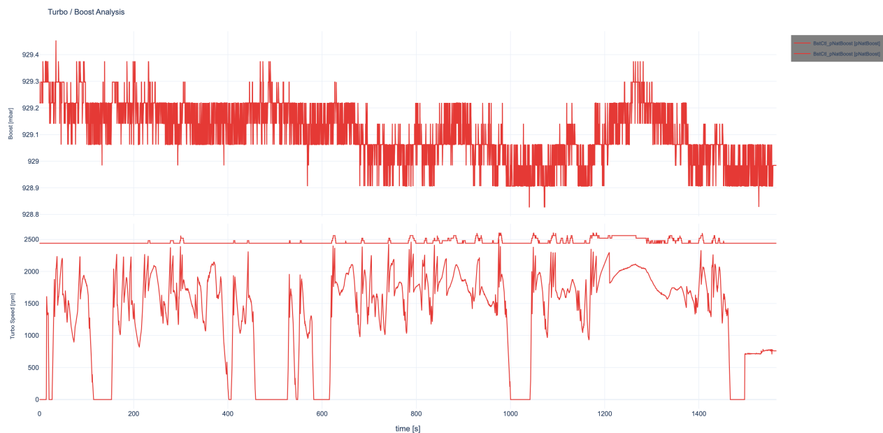
Figure: Turbo / Boost Analysis
