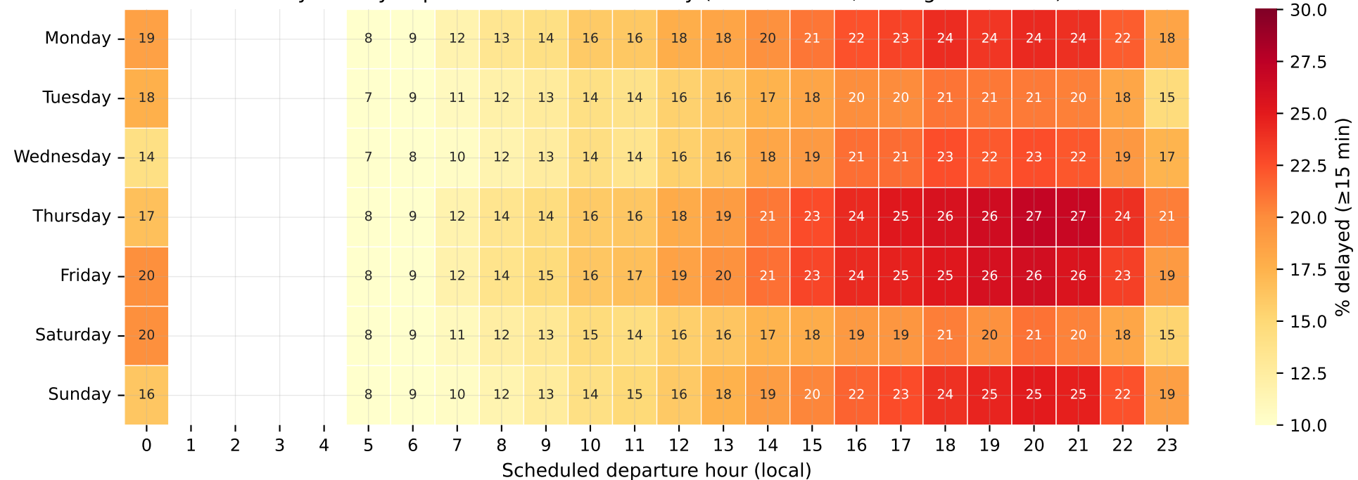
Delay rate by departure hour and weekday (cells with < 1,000 flights masked)
