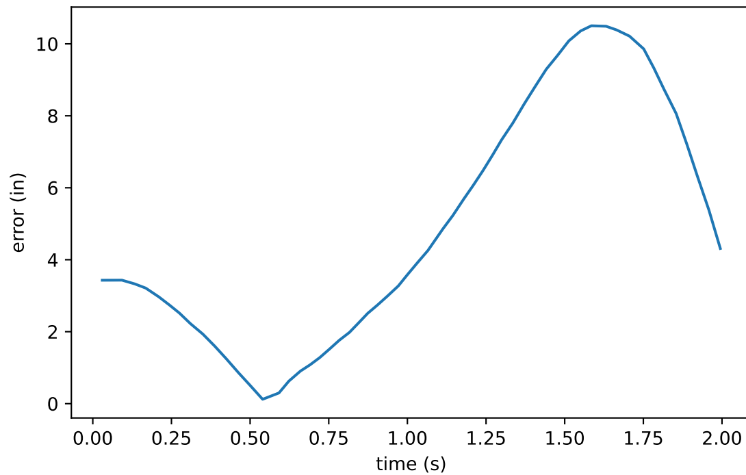
Cross-Track Error
