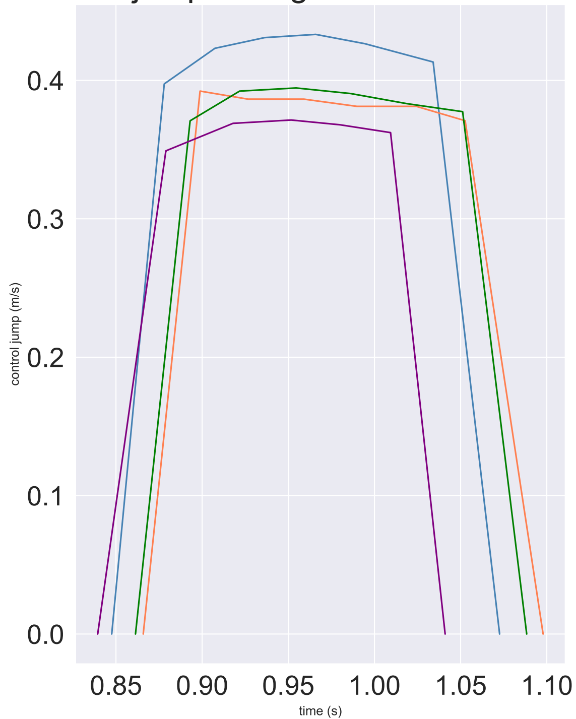
B. Control jump during 200ms handoff interval
