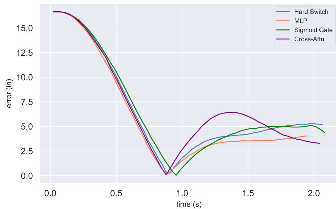
Cross-Track Error
