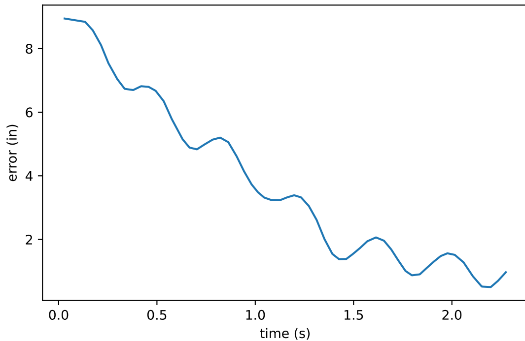
Cross-Track Error
