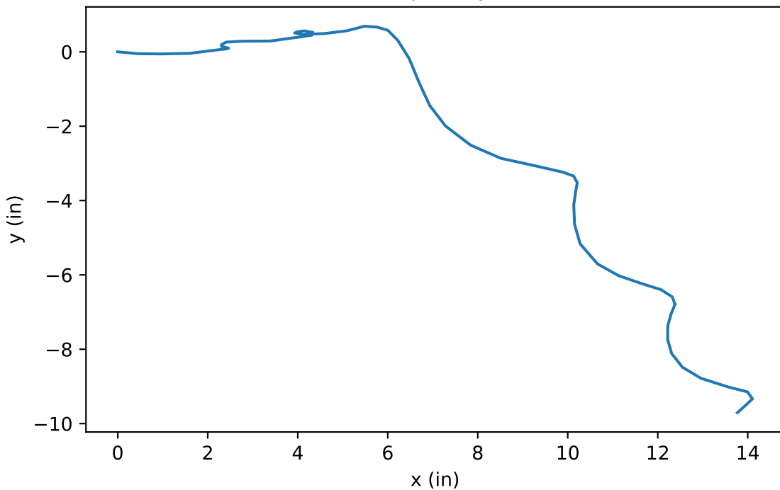
Cross-Track Error
