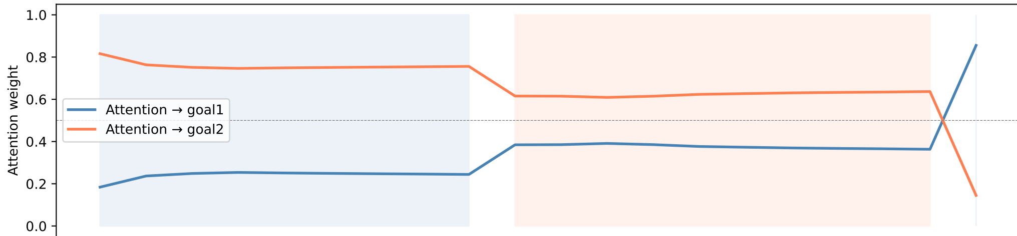
Learned attention tracks active navigation goal
