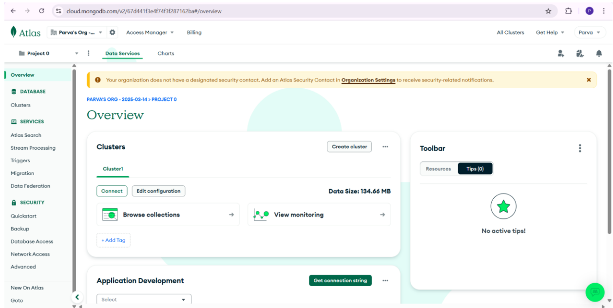
Figure 1: Cluster Created
