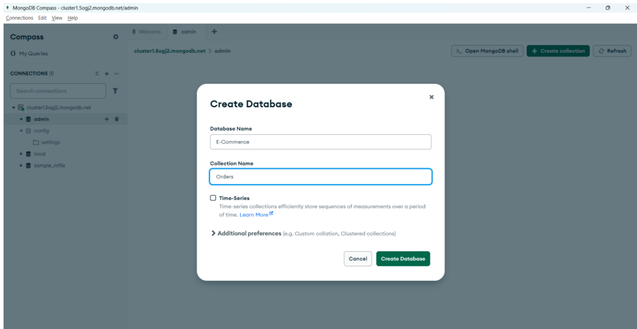
Figure 7: Create Database
