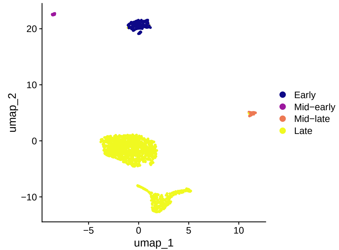
Pseudotime Stage
