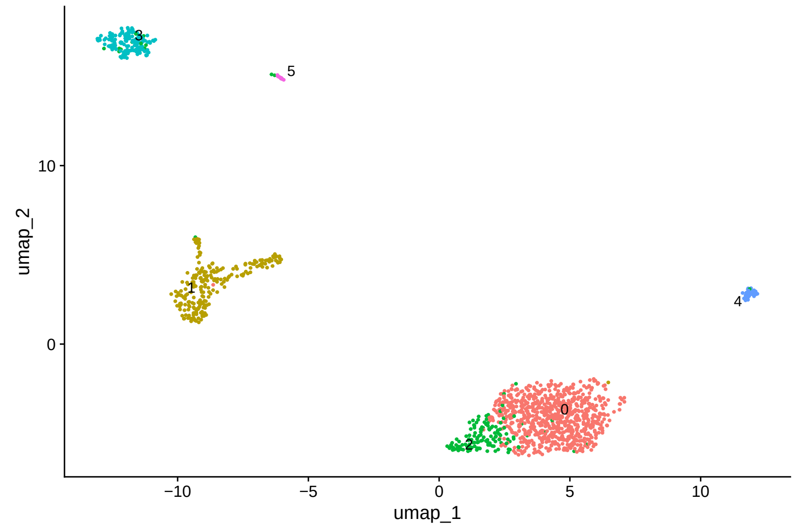
Microglia UMAP by Cluster
