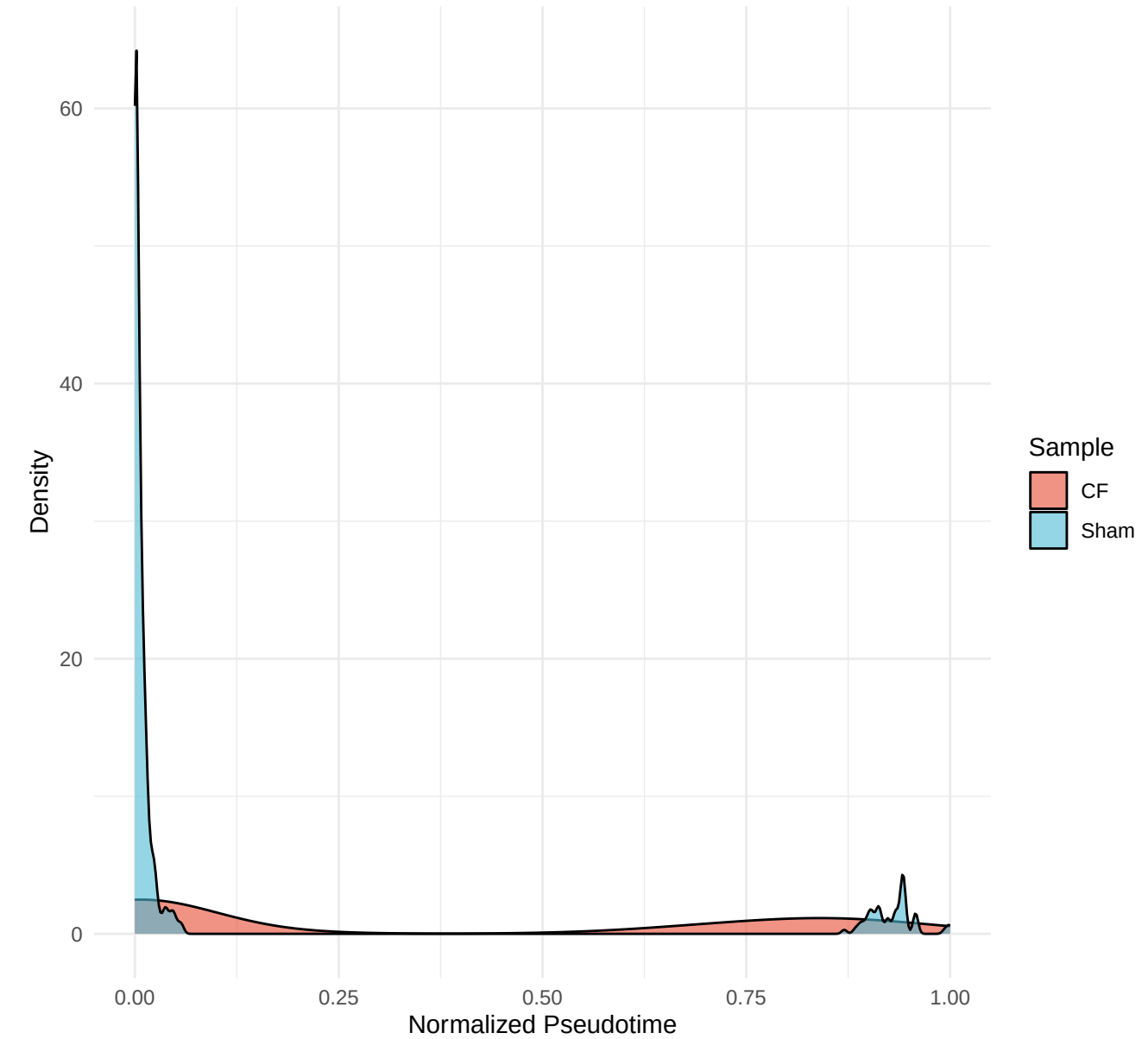
Pseudotime Distribution
