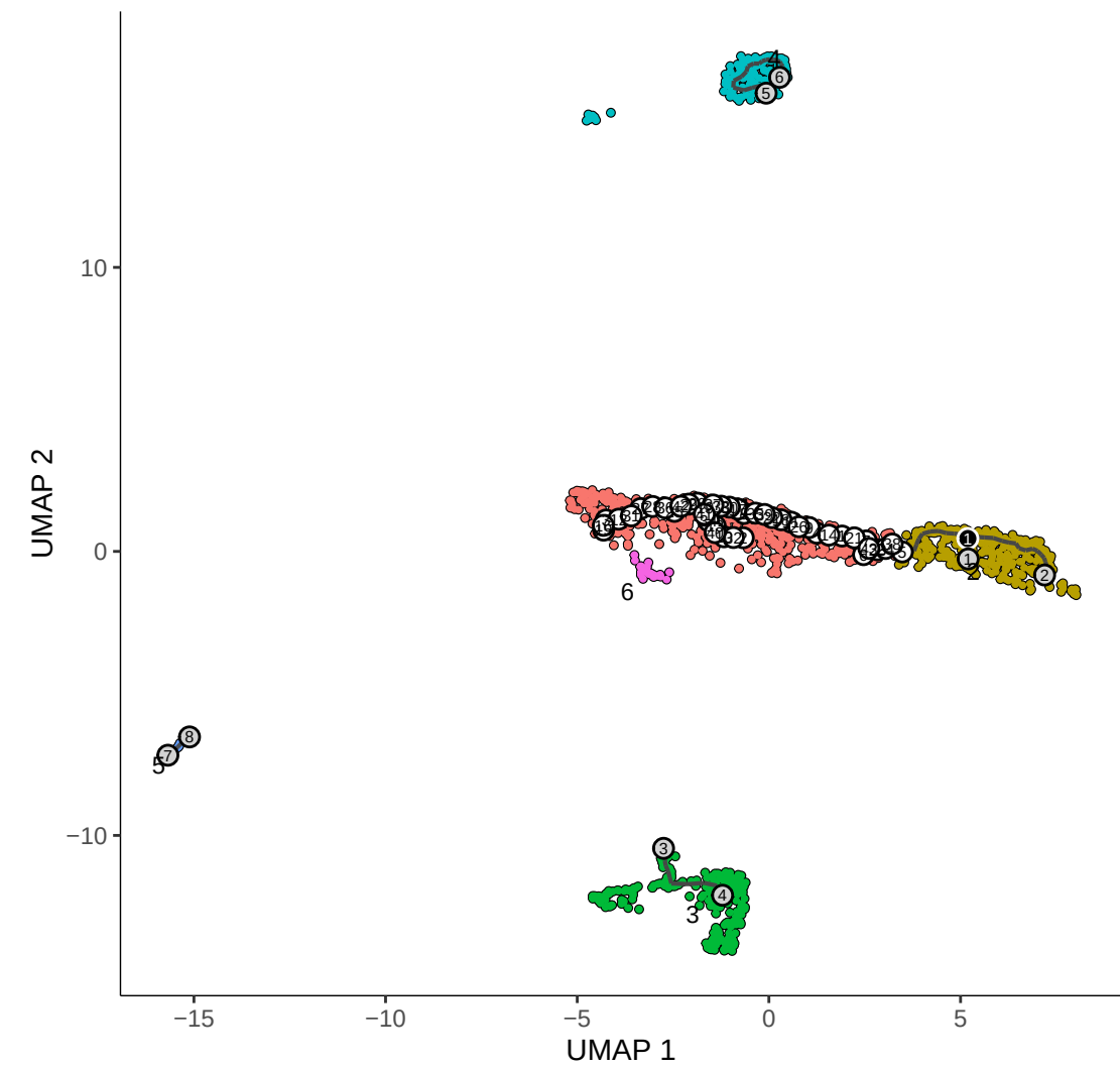
Subclusters
