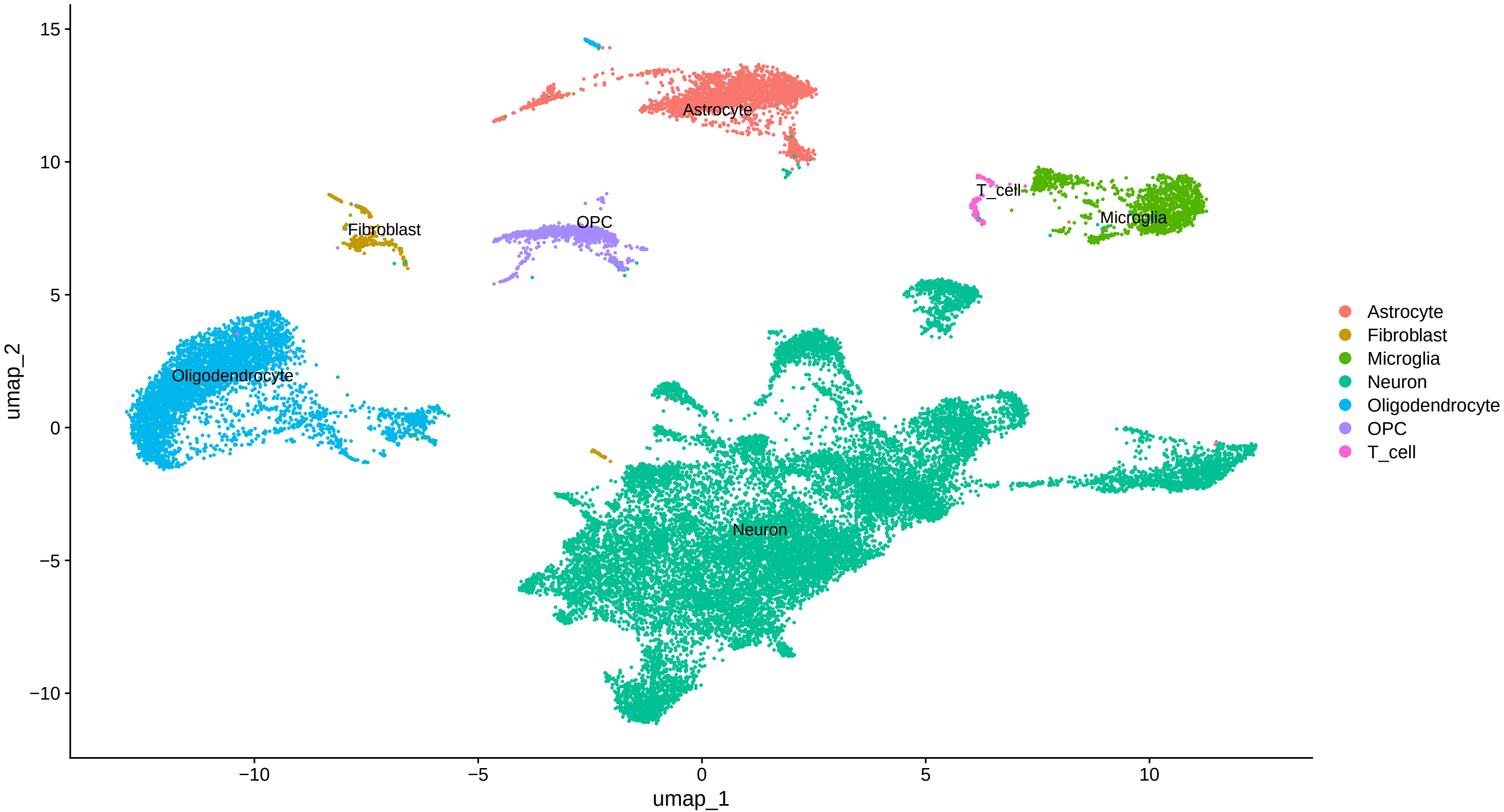
Mouse Hypothalamus: Cell Types
