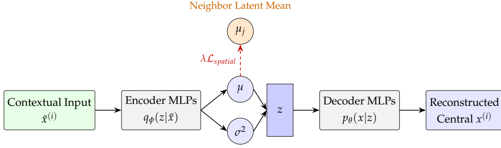
FIGURE 3.2: The proposed Spatial-msiPL architecture. The encoder ingests the contextual vector to map the latent distribution. The spatial coherence penalty explicitly regulates the distance between the central latent mean ( \mu ) and adjacent neighbor means ( \mu_j ). The decoder reconstructs only the isolated central spectrum.
