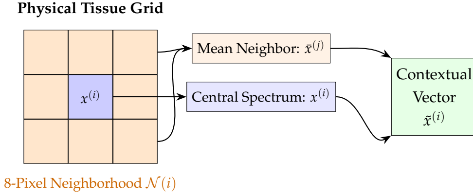
FIGURE 3.1: Generation of the contextual input vector \tilde{x}^{(i)} . The central spectrum (blue) is isolated, while the surrounding 8-pixel Moore neighborhood (orange) is averaged. Both are concatenated to form the 1D spatial input.
