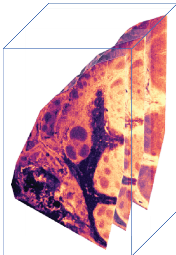
FIGURE 2.1: A representation of the high-dimensional mass spectrometry imaging data hypercube. The 3D bounding box illustrates how 2D spatial tissue planes stack across the mass-to-charge ( m/z ) spectral dimension. Adapted from [Aspect Analytics 2026].
