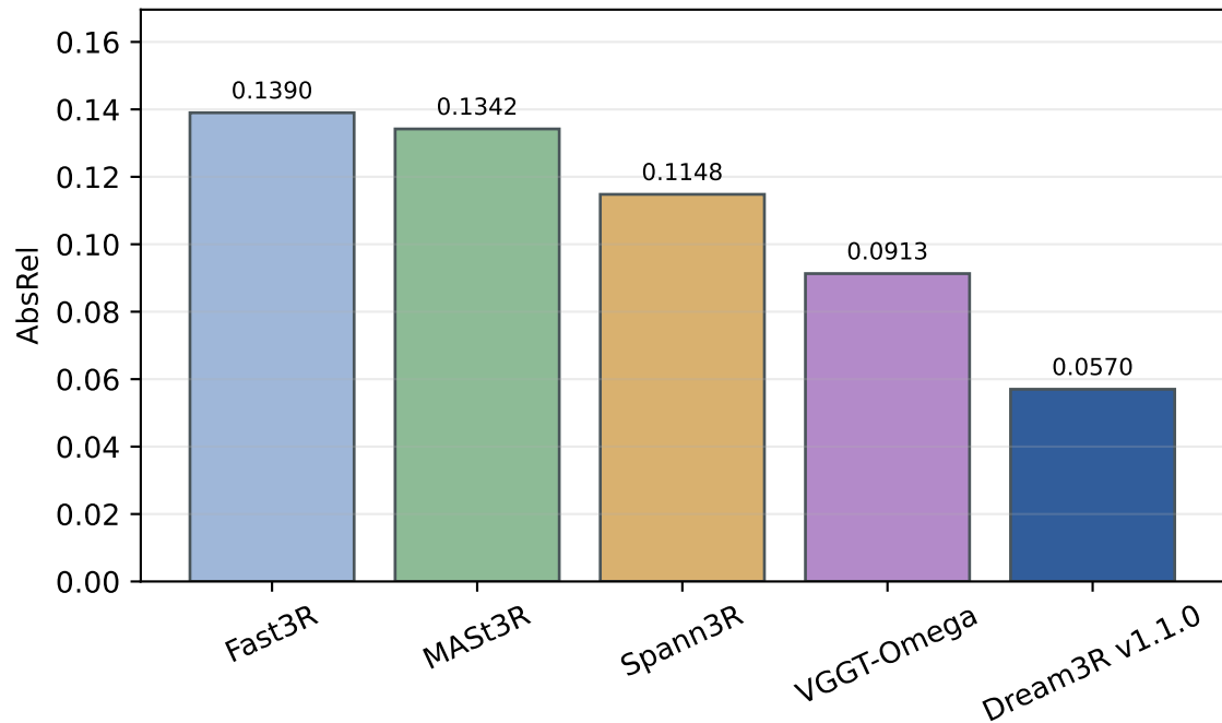
ETH3D
