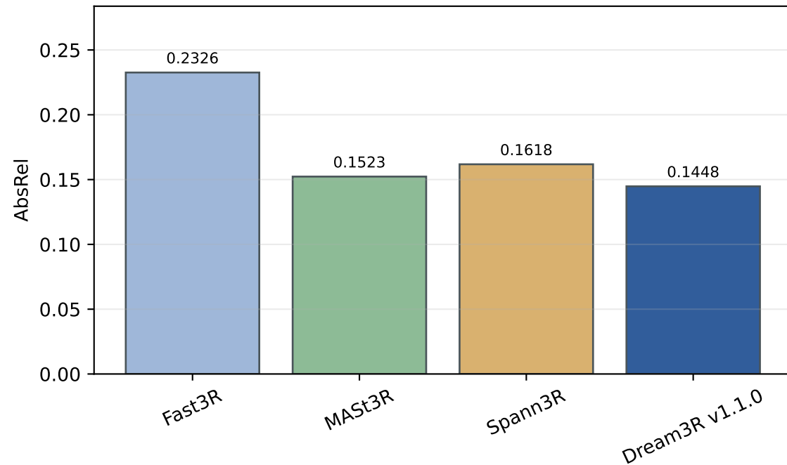
KITTI
