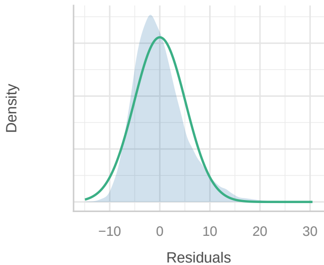
Figure 4: Final model diagnostic plots
