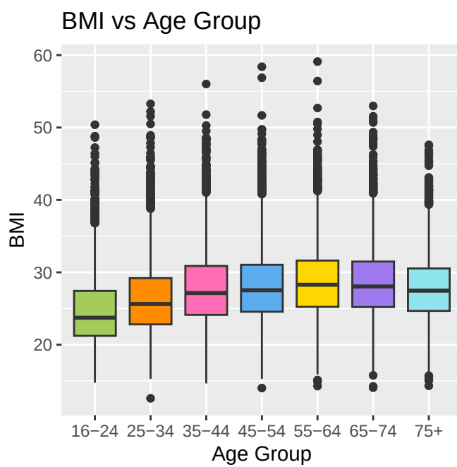
Figure 3: Boxplots for the demographic variables, age group and sex
