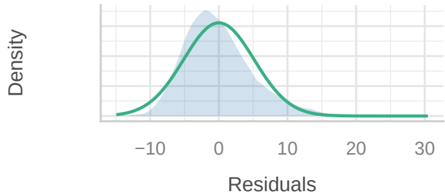
Figure 6: Final model diagnostic plots
