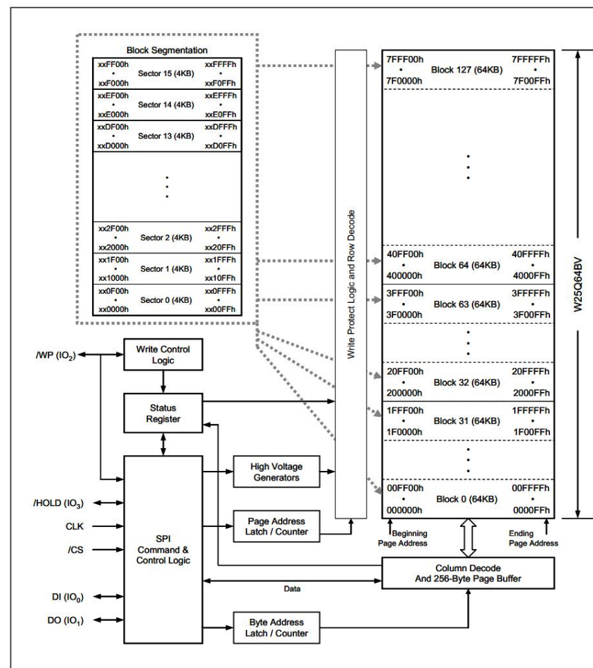
Figure 2. W25Q64BV Serial Flash Memory Block Diagram
