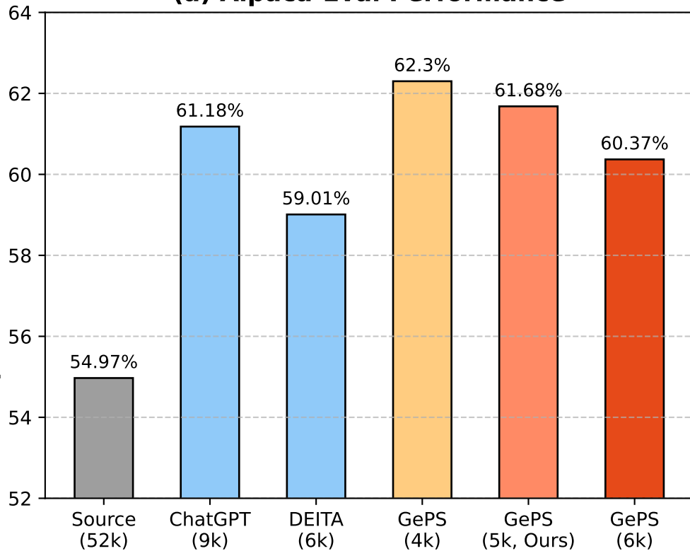
(a) Alpaca-Eval Performance
