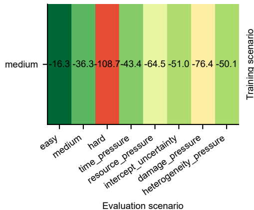
hungarian damage
