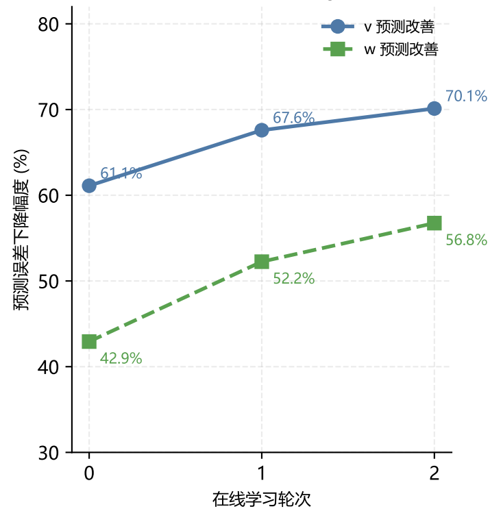
(a) 50ms延迟 0-GP-MPC (Non-T, Update)
