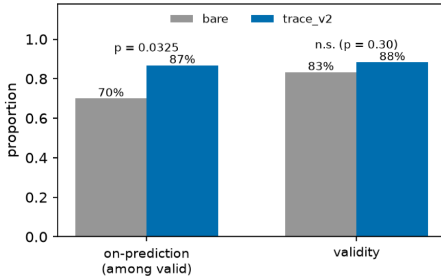
Figure 3. Bare versus trace_v2 , by cell and pooled. Caption caveat: the bars pool the bare arm's two collection waves, which §6.4 shows drift materially, so the pooled bare bar is a mixture; the same-wave comparison in §6.4 is the wave-controlled picture.
