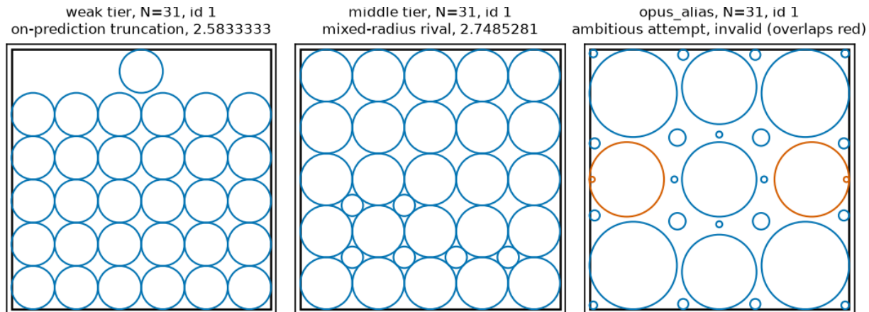
Figure 3: Three attractor families at a single cell, N = 31 . One representative packing per tier, ledger sample id in each panel title (weak tier bare id 1, on-prediction truncation 2.5833333; middle tier sonnet_bare id 1, mixed-radius rival 2.7485281; opus_alias id 1, invalid, with only the offending circles highlighted). Source: arm_f_candidates_v2.jsonl via fig_scripts.py , deterministic (the exemplar rows’ geometry is byte-identical in v1; v2 differs only in provenance metadata).
