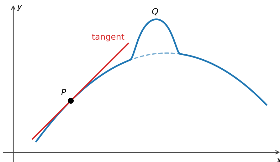
Figure 15.2: Changing the curve away from P (solid) does not change the tangent at P : the original curve (dashed) and the modified one agree near P .
