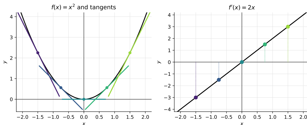
Figure 15.6: Left: f(x) = x^2 with its tangents at several points. Right: the derivative f'(x) = 2x . The height of each dot on the right is the slope of the tangent of the same color on the left.
