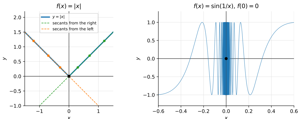
Figure 15.4: Two curves without a tangent at the origin. Left: for |x| , secants from the right are all the line y = x , secants from the left are all the line y = -x . Right: the graph of \sin(1/x) (with value 0 at x = 0 ) near the origin.
