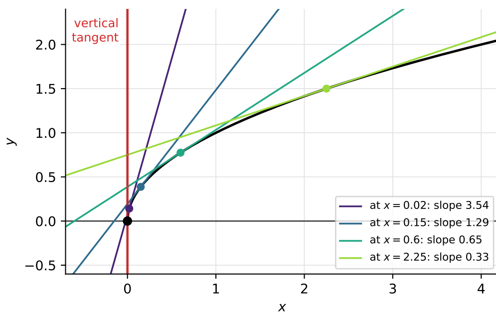
Figure 15.7: Tangents to y = \sqrt{x} with slopes 1/(2\sqrt{x}) . As the point of tangency approaches 0 the tangents become steeper without bound; at the origin the tangent is vertical and \sqrt{x} is not differentiable.
