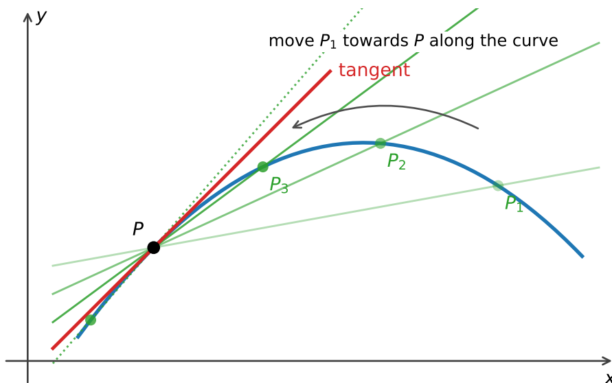
Figure 15.3: As P_1 moves along the curve towards P , the secants through P and P_1 approach the tangent at P . The limiting position should not depend on the side from which P_1 approaches P .
