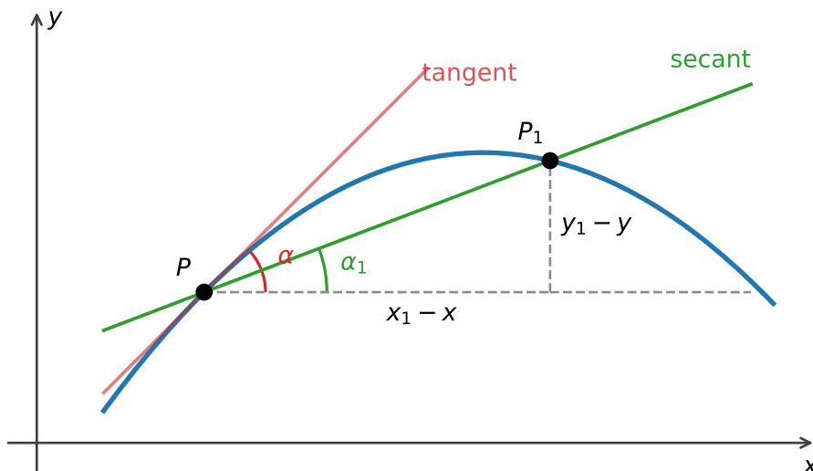
Figure 15.5: The secant through P = (x, y) and P_1 = (x_1, y_1) forms a right triangle with legs x_1 - x and y_1 - y , so \tan(\alpha_1) = (y_1 - y)/(x_1 - x) .
