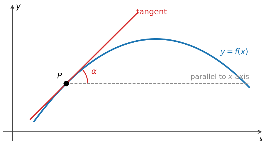
Figure 15.1: The tangent at P is completely characterized by the angle \alpha it makes with the line through P parallel to the x -axis.
