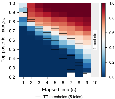
a DQN greedy action on test states
