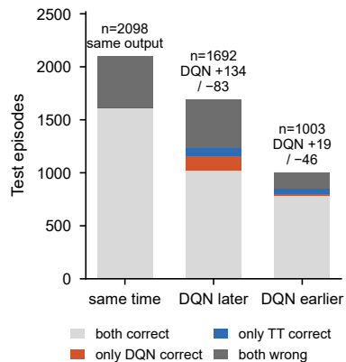
c Paired outcome, TT vs DQN
