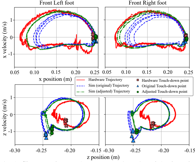
Fig. 3: Sim-to-real gap : Phase-space trajectories of the front feet.
