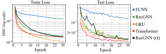
Fig. 5: Loss trajectories. (Left) Training loss for different NN architectures. (Right) Test loss evaluated during training.
