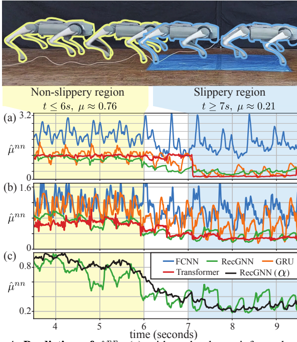
Fig. 4: Prediction of \hat{\mu}^{nn} : (a) without hardware-informed model matching, (b) with hardware-informed model matching, and (c) with \alpha -scaling.
