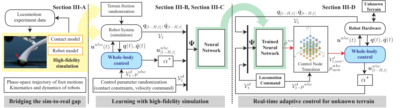
Fig. 2: Overall architecture: Using simulation, we train an NN that infers the terrain friction coefficient through supervised learning. Based on the inferred friction coefficient, the robot adapts its locomotion behavior in response to terrain properties.
