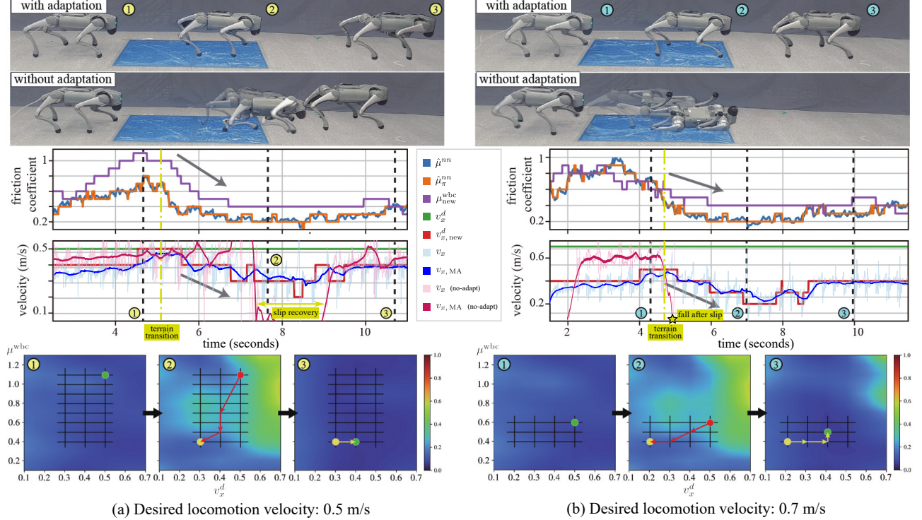
Fig. 6: Hardware experiments for adaptive locomotion: The first, second, and third rows illustrate the experiment snapshots, the trajectories of control parameters, and the control parameter adjustments induced by the cost updates. Measured velocity was smoothed using a 0.3-s moving-average window.
