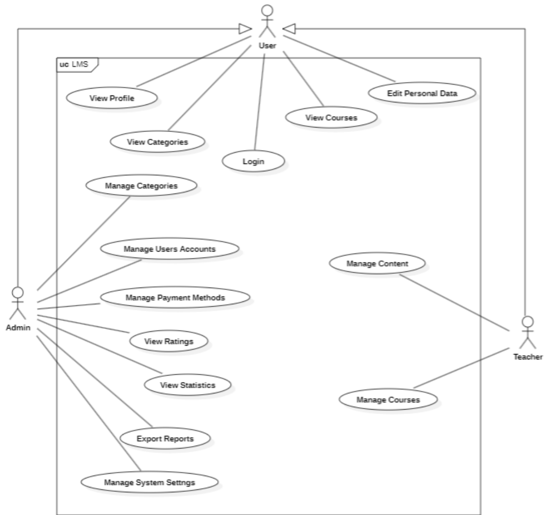
Figure (4.2) Use Case Diagram for Current Project
