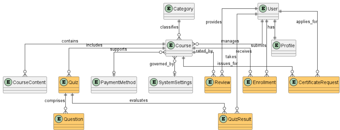
Figure (5.2) ERD
