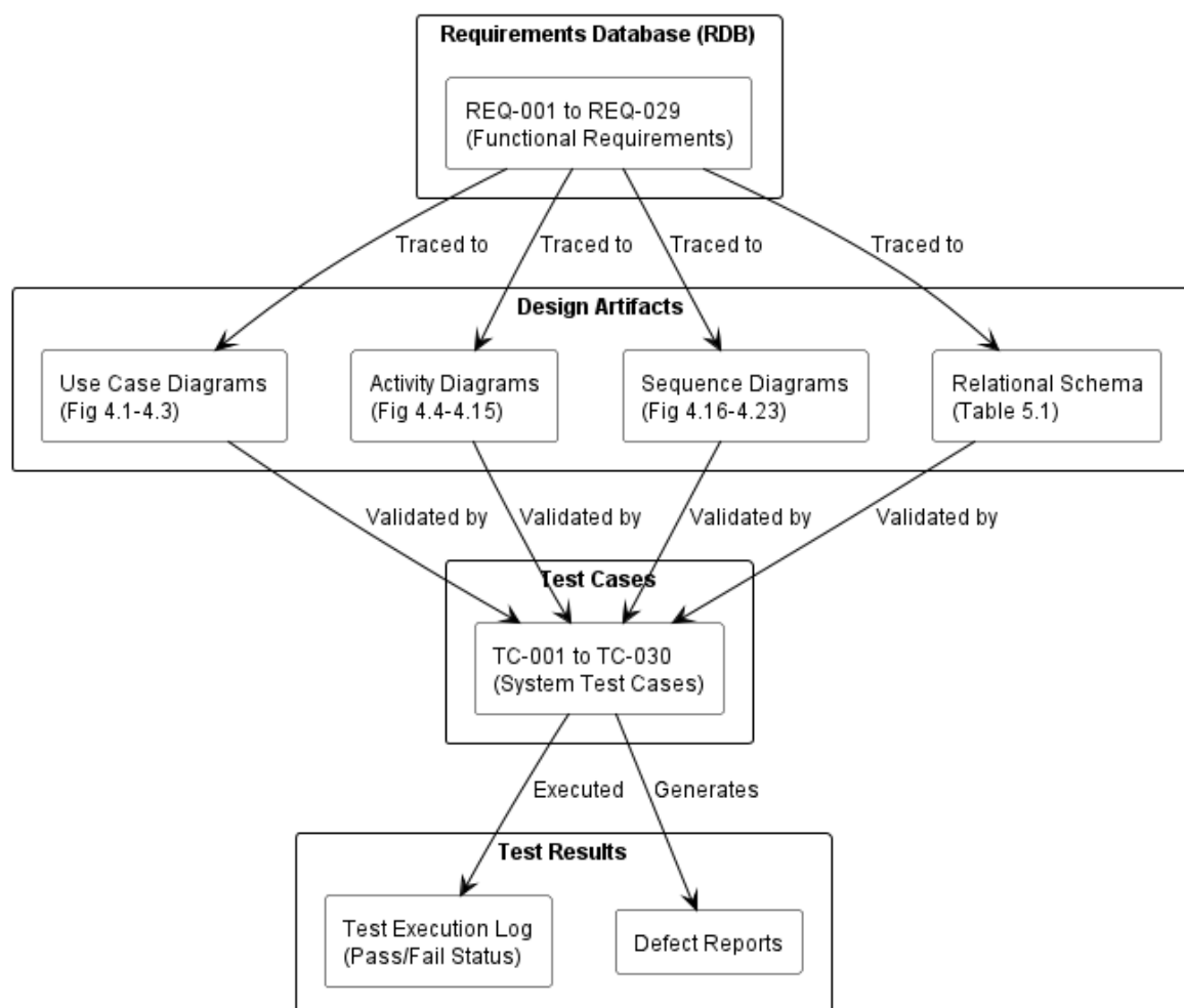
Figure (7.1) Test Case Traceability Diagram
