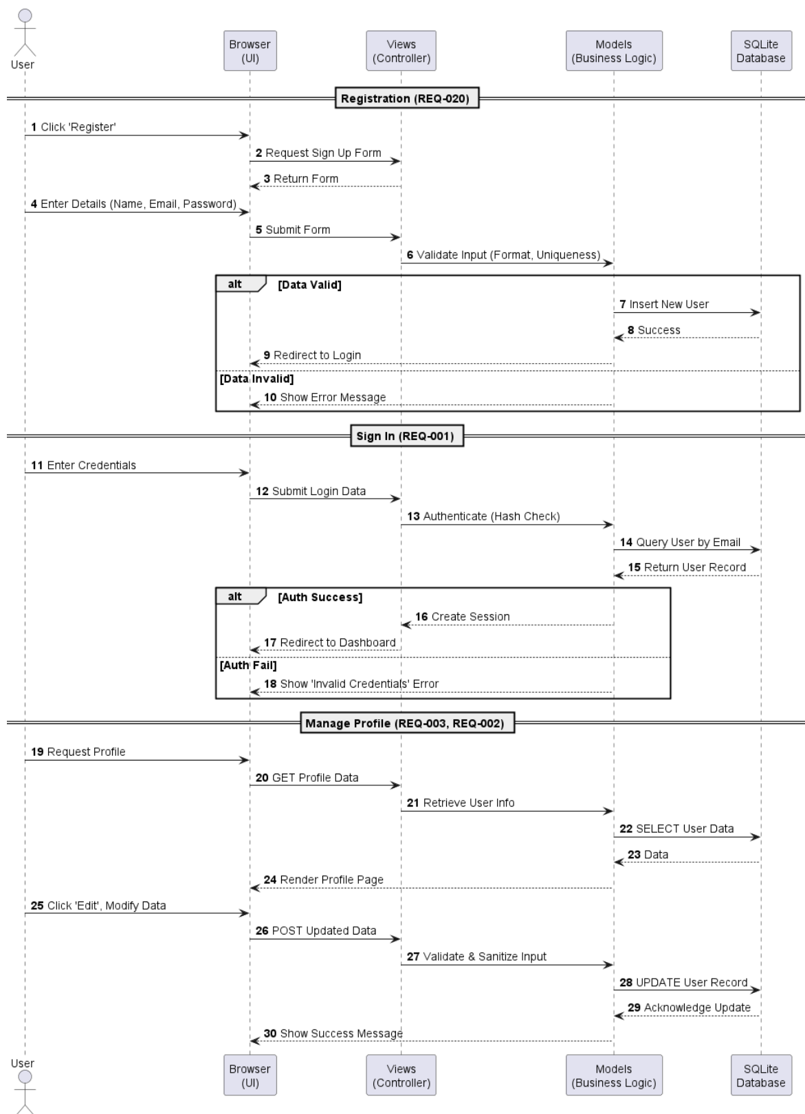
Figure (4.17) Sequence Diagram for Authentication and Profile Management
