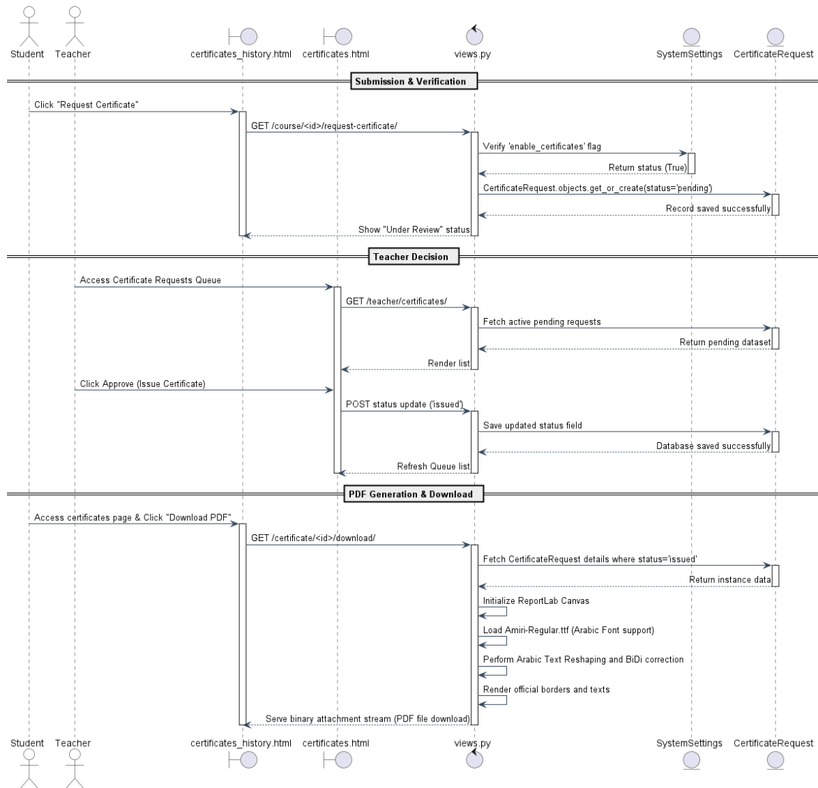
Figure (4.24) Sequence Diagram for Certificate Verification & Generation
