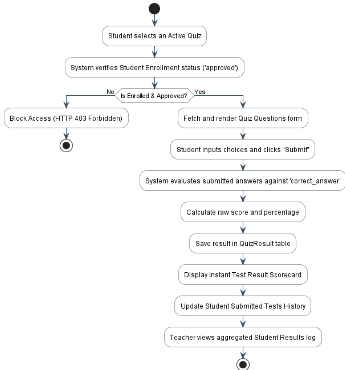
Figure (4.14) Testing Application & Automatic Grading
