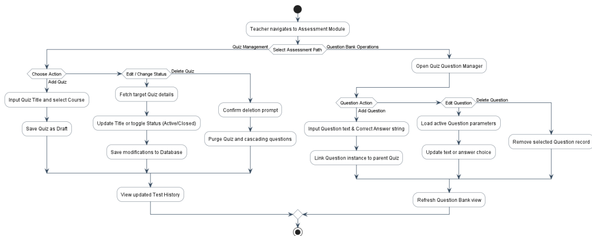
Figure (4.12) Quiz & Questions Management
