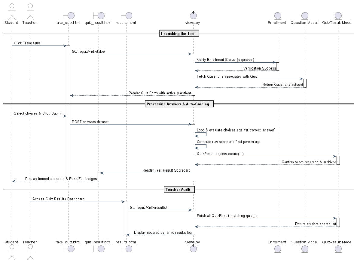
Figure (4.22) Sequence Diagram for Examination & Auto-Grading
