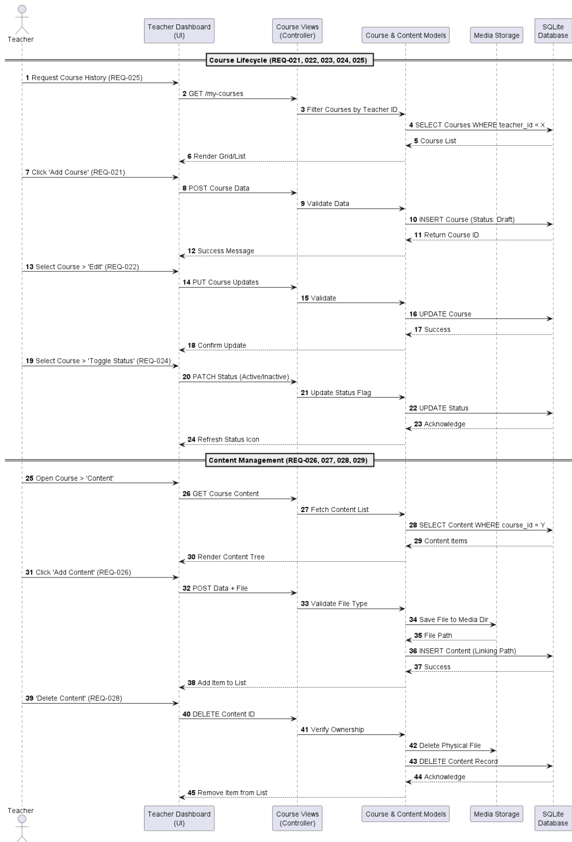
Figure (4.19) Sequence Diagram for Course and Content Management
