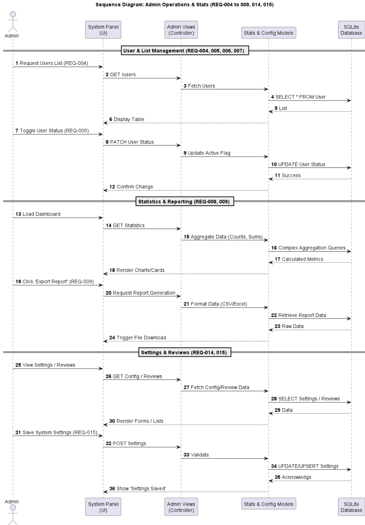
Figure (4.20) Sequence Diagram for Admin Operations and Stats
