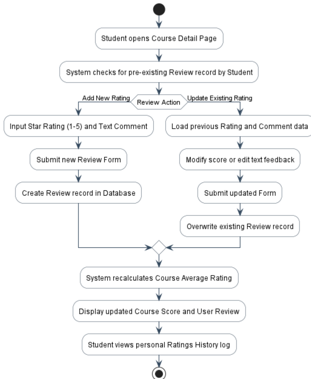
Figure (4.16) Course Ratings & Reviews Management
