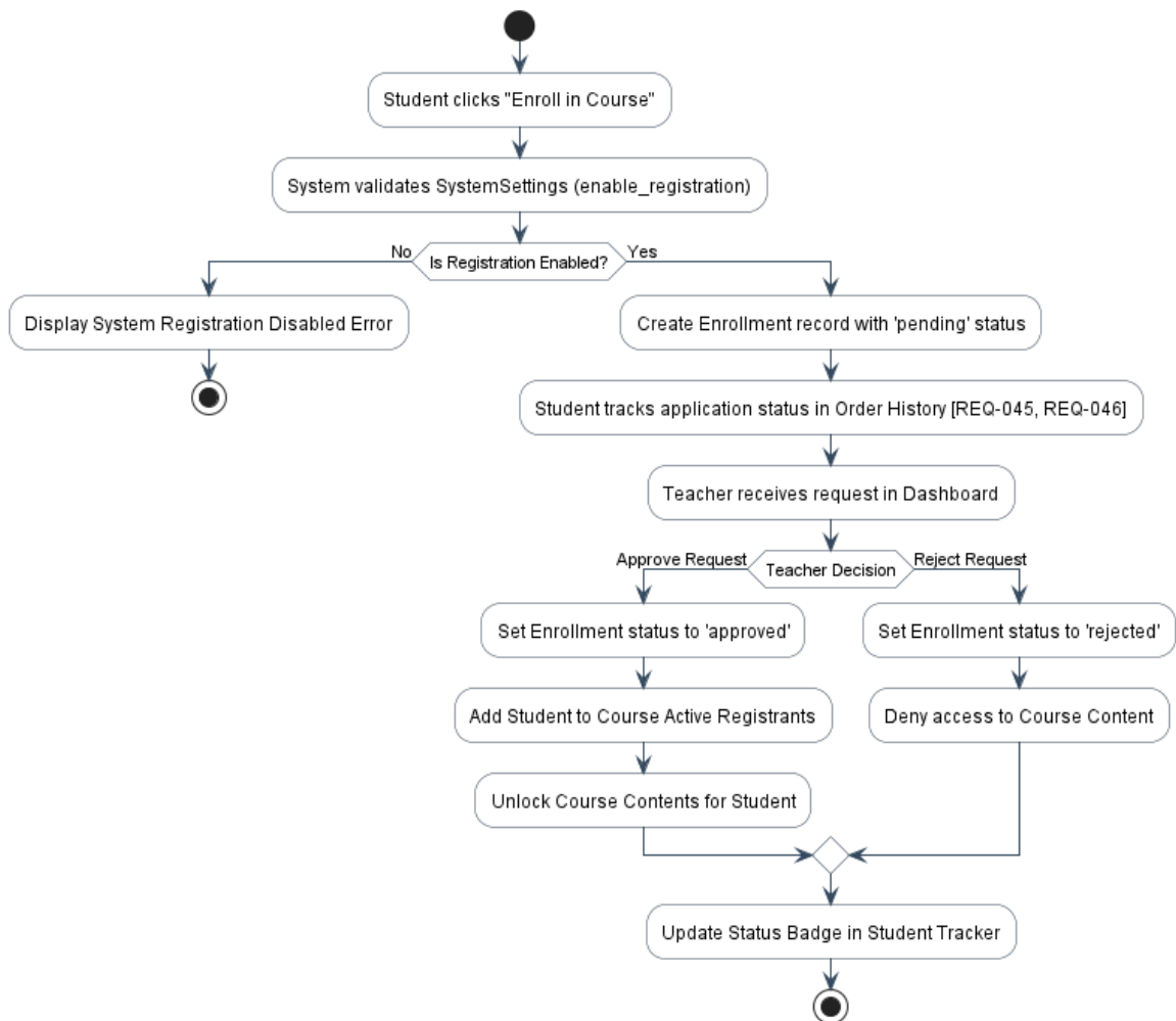
Figure (4.13) Enrollment Request & Tracking Workflow
