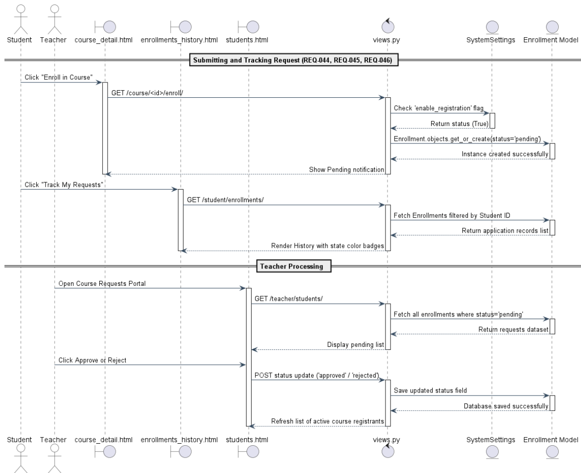
Figure (4.23) Sequence Diagram for Registration Request & Tracking
