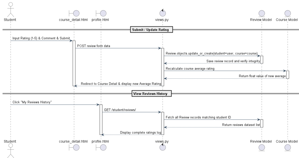
Figure (4.25) Sequence Diagram for Course Rating & Review
