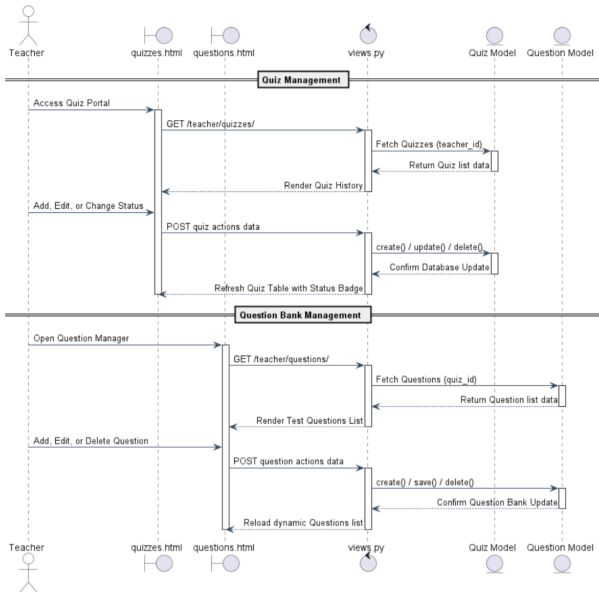
Figure (4.21) Sequence Diagram for Quiz & Question Management
