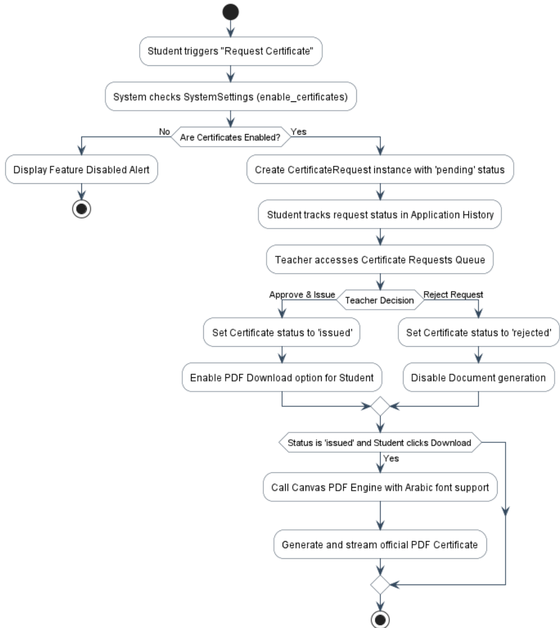
Figure (4.15) Certificate Request & PDF Generation Workflow
