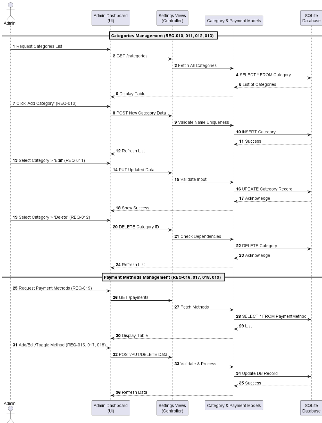
Figure (4.18) Sequence Diagram for Categories and Payment Methods Management
