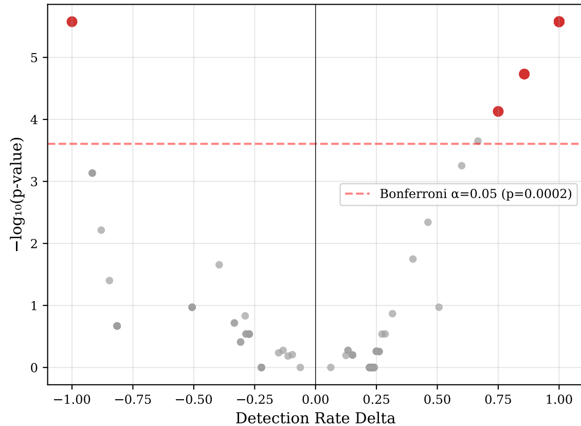
C5: Volcano Plot — Token Effect Size vs Significance
