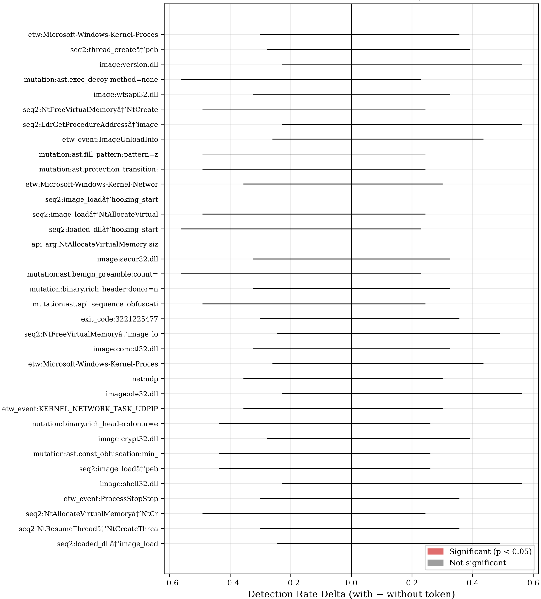
C5: Counterfactual Token Attribution (Forest Plot)
