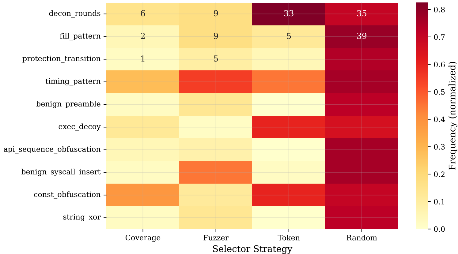
AST Mutation Selection Frequency by Selector
