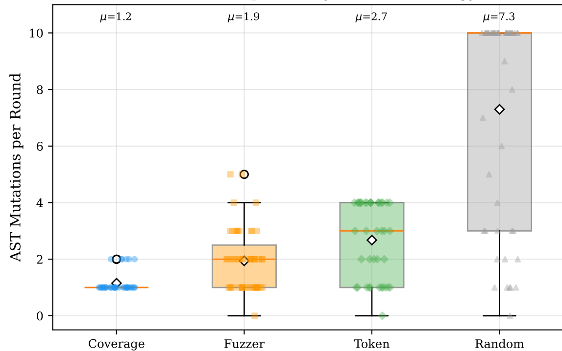
Mutation Recipe Size by Selector Strategy
