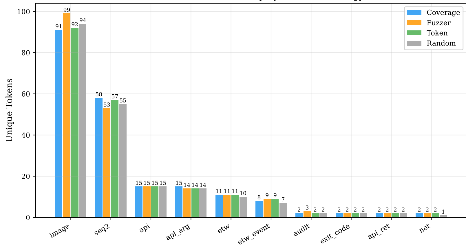
Behavioral Token Diversity by Selector Strategy
