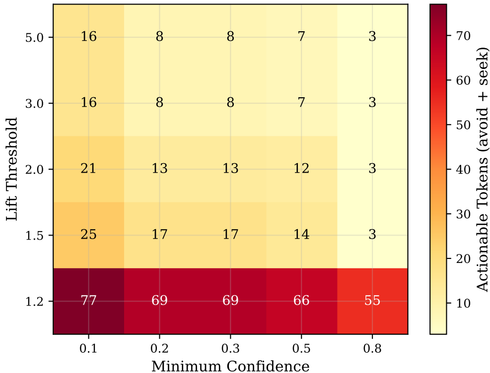
C1: Actionable Token Count by Scoring Parameters
