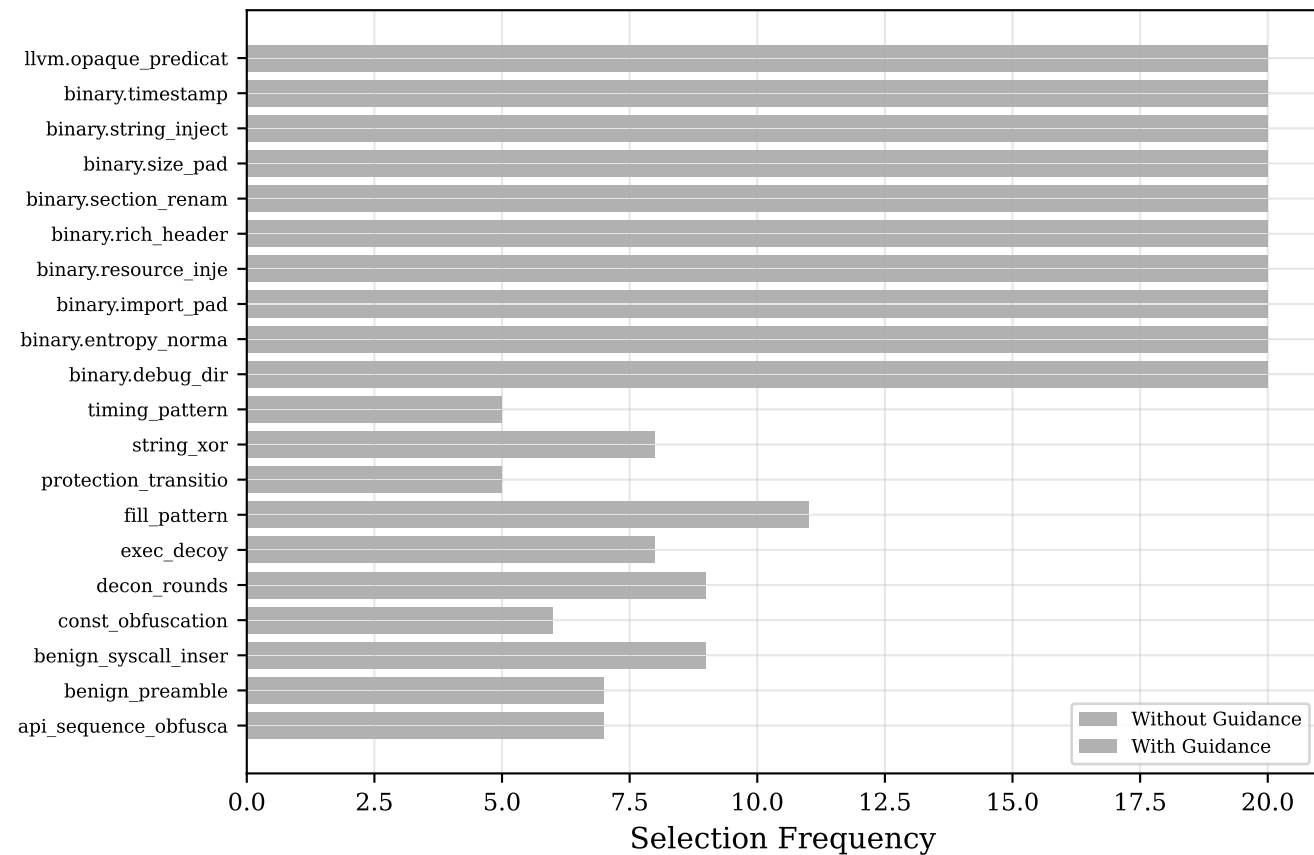
Random
