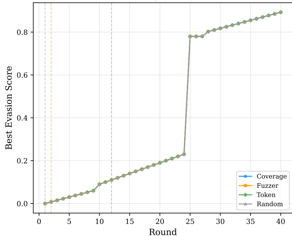
Score Convergence by Selector
