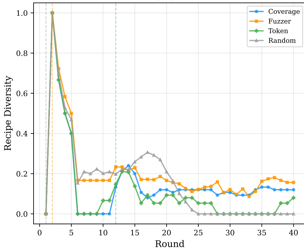
Diversity by Selector
