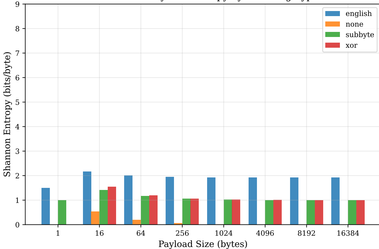
I1: Encoded Payload Entropy by Encoding Type
