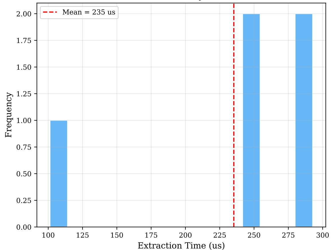
I7: Extraction Latency Distribution
