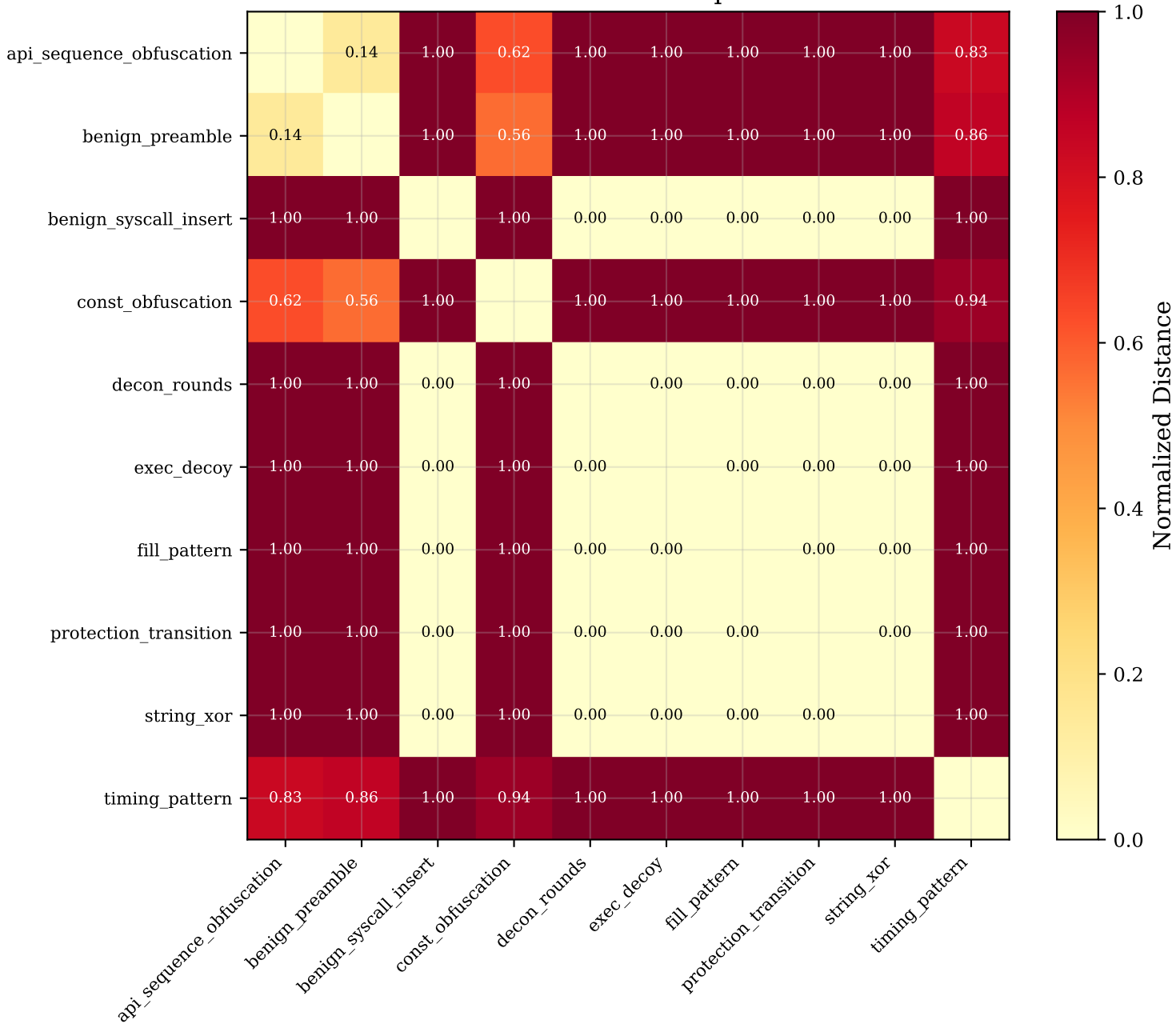
I9: Pairwise Mutation Output Distance
