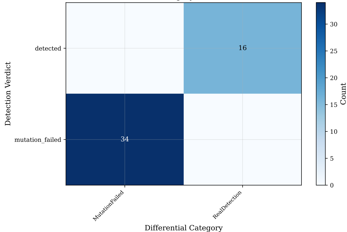
B2: Verdict \rightarrow Category Confusion Matrix
