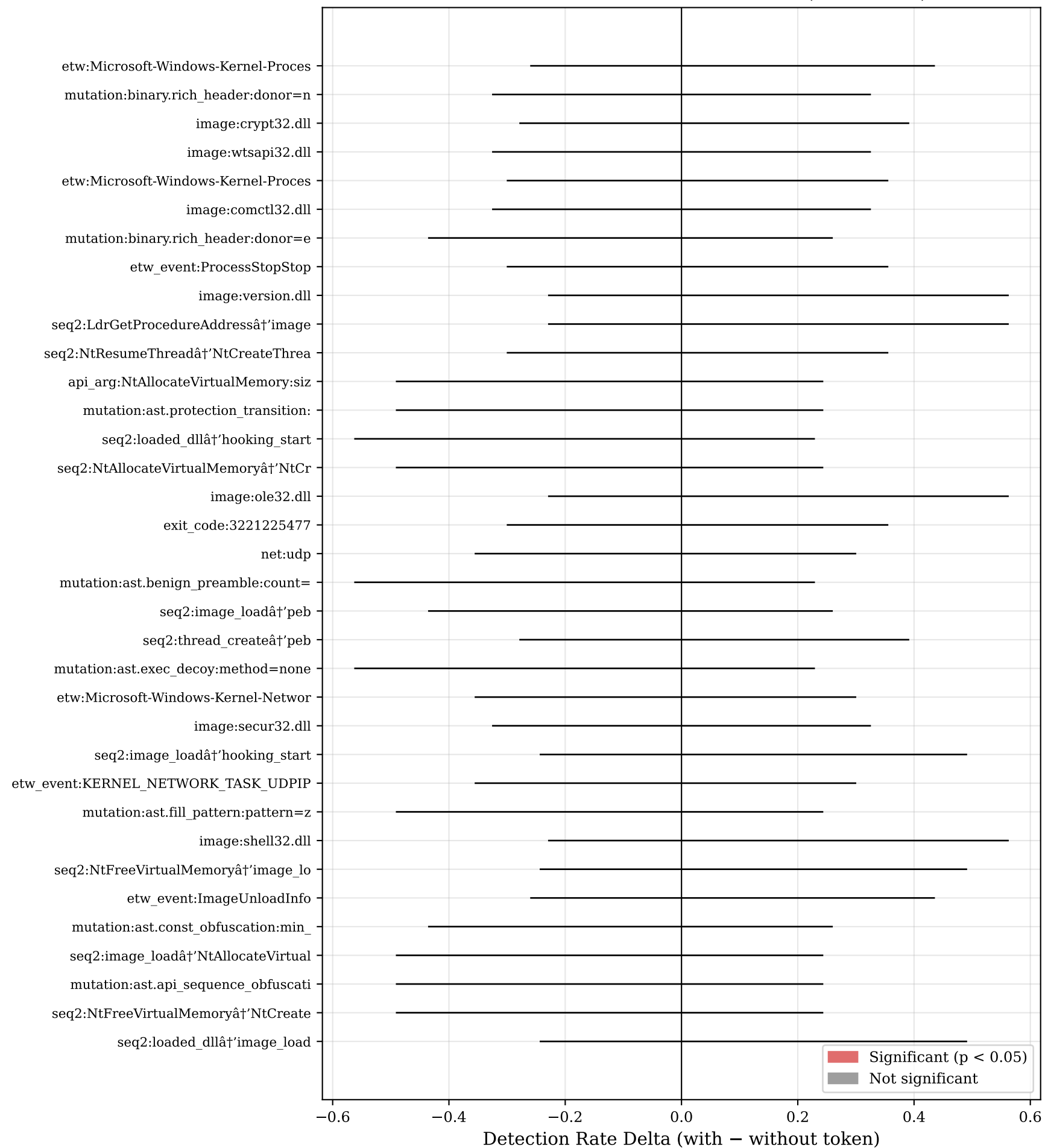
C5: Counterfactual Token Attribution (Forest Plot)
