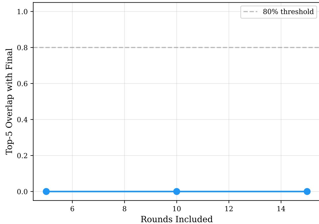
C4: Token Ranking Convergence
