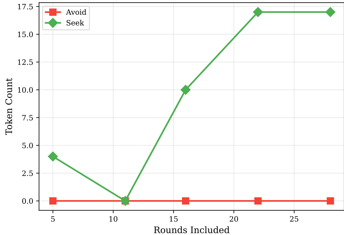
I10: Guidance Token Counts over Rounds
