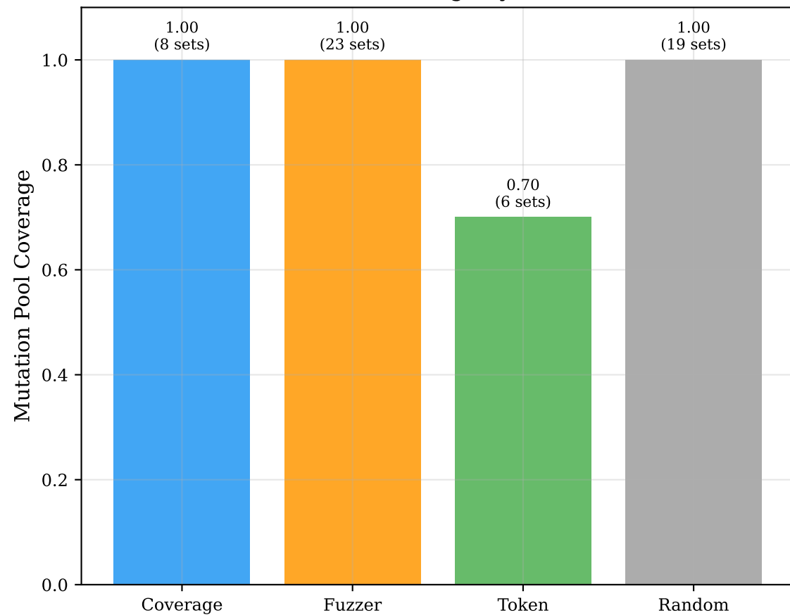
I11: Pool Coverage by Selector
