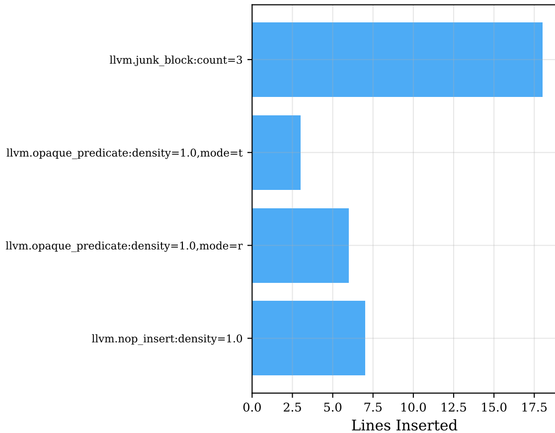
I3: IR Mutation Insertions
