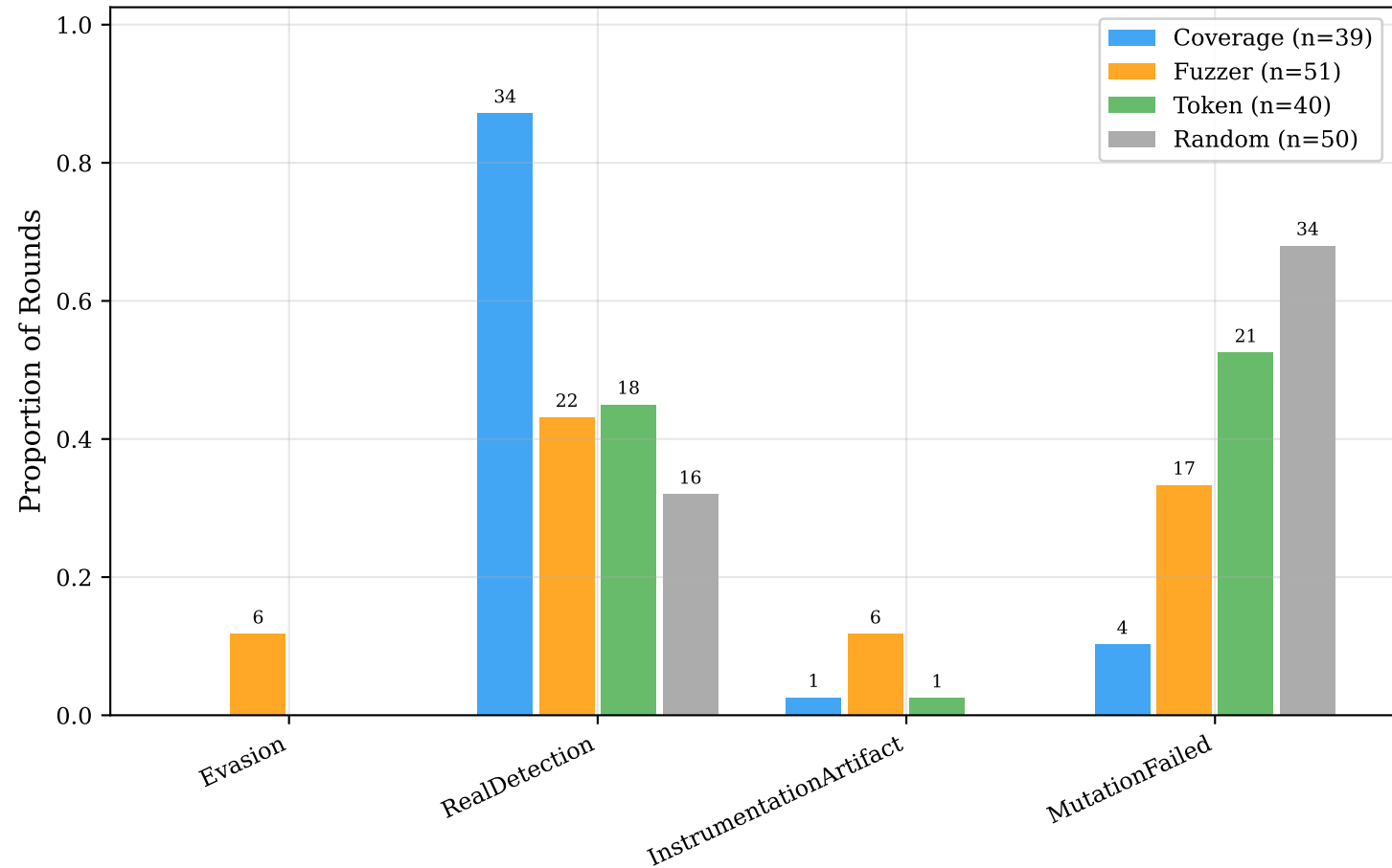
Outcome Distribution by Selector Strategy
