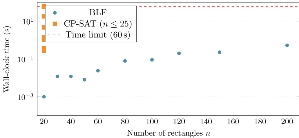
Figure 3: Solve time (log scale) for BLF and CP-SAT. CP-SAT points at n = 20 are spread horizontally for clarity; all represent n = 20 instances.
