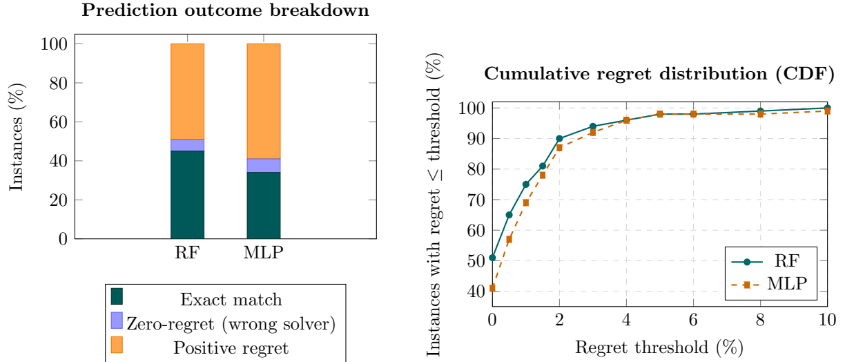
Figure 6: ML model comparison on 100 held-out test instances (seed=999). Left : outcome breakdown — exact match means the predicted solver equals the oracle; zero-regret/wrong means the predicted solver achieves the same height as the oracle but is a different solver. Right : cumulative distribution of relative regret (H_{\text{pred}} - H_{\text{oracle}})/H_{\text{oracle}} \times 100\% . RF dominates MLP at all thresholds up to 3%, but both models keep regret below 2% on \geq 87\% of instances.
