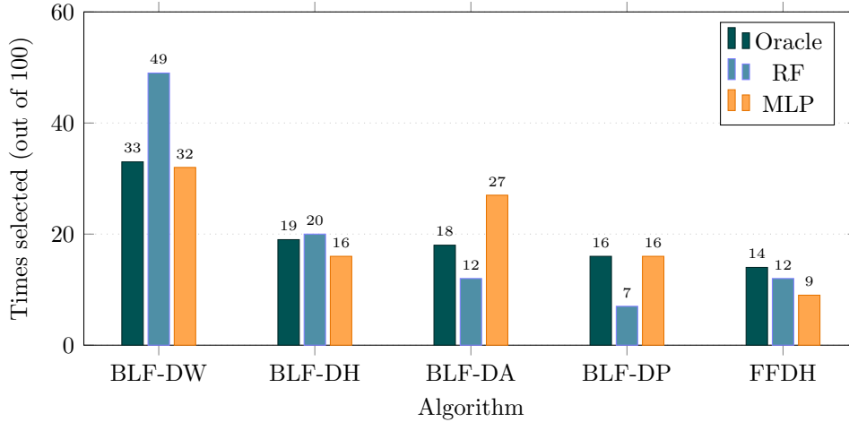
Figure 5: Algorithm selection frequency on 100 test instances: oracle (true best performer) vs. RF vs. MLP predictions. RF over-selects BLF-DW (49 vs. 33 actual) and severely under-selects BLF-DP (7 vs. 16), biasing towards width-sorted BLF. MLP over-selects BLF-DA (27 vs. 18 actual) and under-selects FFDH (9 vs. 14), reflecting different learned feature interactions. No model ever selects any Skyline variant.
