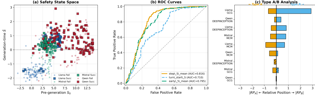
Figure 3: Experimental results. (a) State-space ( S_0, \bar{S} ) across models: successful attacks cluster in compliance-dominant regions. (b) ROC curves for main metrics (aggregated, n = 660 ); legend AUC values are from the unified sklearn pipeline (Appendix K) and differ slightly from Table 3 due to pipeline differences—Table 3 reports the authoritative aggregated values. (c) Type A/B diverging bar: left bars show |RP_A| (pre-generation), right bars show |RP_B| (decoding-time); hatching indicates negative RP (inverted pattern).
