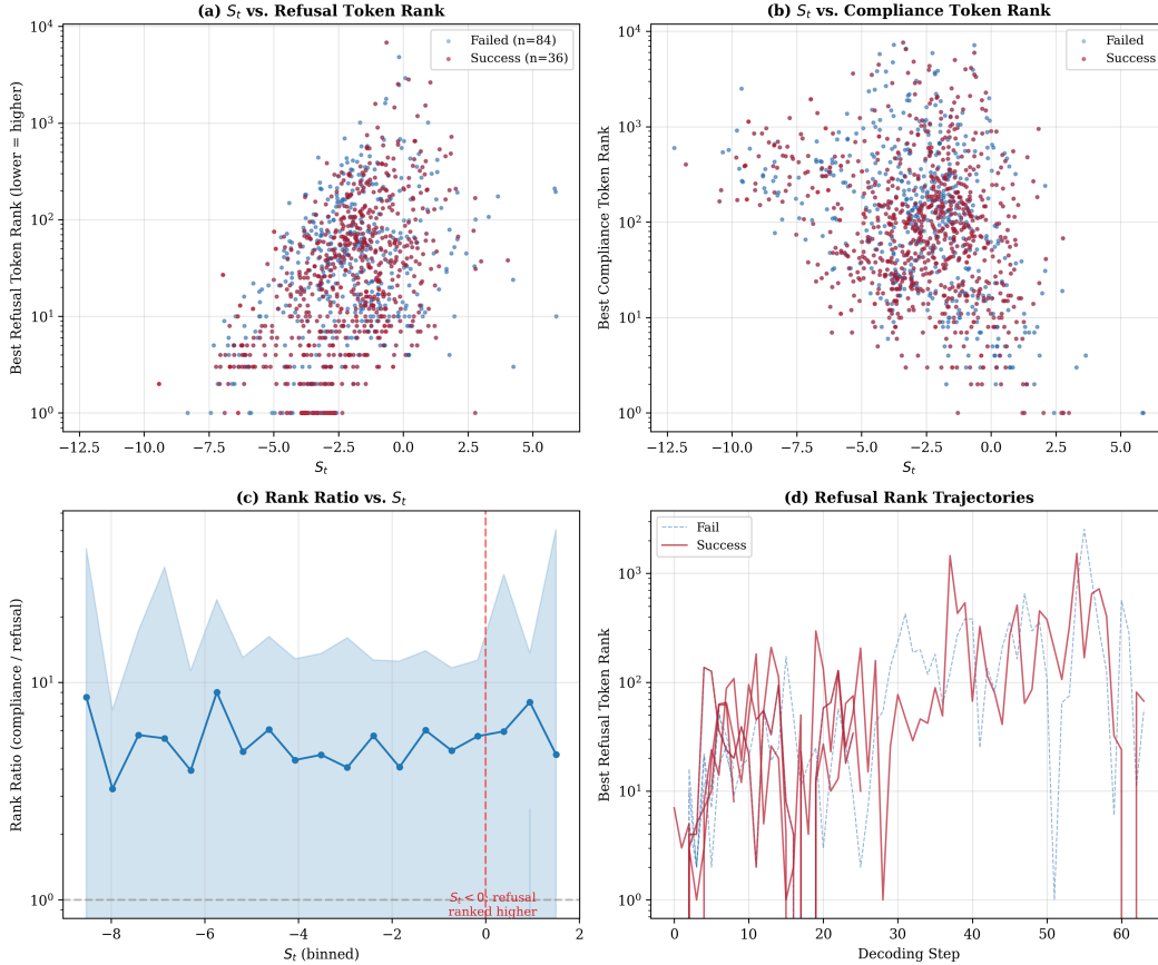
Figure 10: Token rank linkage. (a) S_t vs. best refusal token rank: negative S_t corresponds to refusal tokens in top-10; positive S_t pushes them to rank > 100 . (b) Inverse pattern for compliance tokens. (c) Rank ratio confirms monotonic relationship. (d) Per-sample refusal rank trajectories: successful jailbreaks (red) maintain high refusal ranks throughout.
