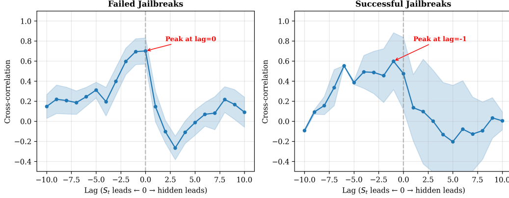
Figure 11: Lead/lag analysis. Cross-correlation between S_t and hidden-state refusal projection. Left: failed jailbreaks peak at lag=0 (simultaneous). Right: successful jailbreaks peak at lag=-1 ( S_t leads hidden by 1 step).
