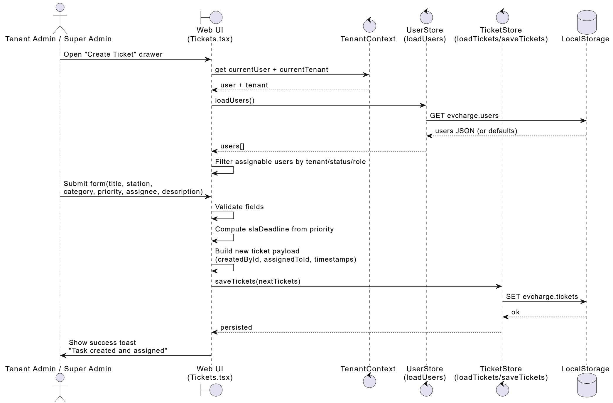
EV Charge DZ - Sequence Diagram (Current App Flow: Create and Assign Ticket)
