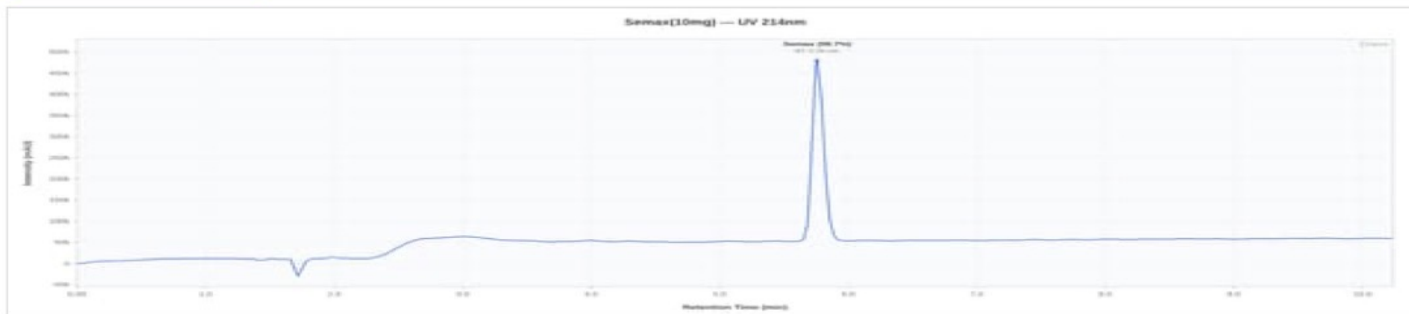
Semax 10mg - 20260507-XA10-2CF1: UV Chromatogram
